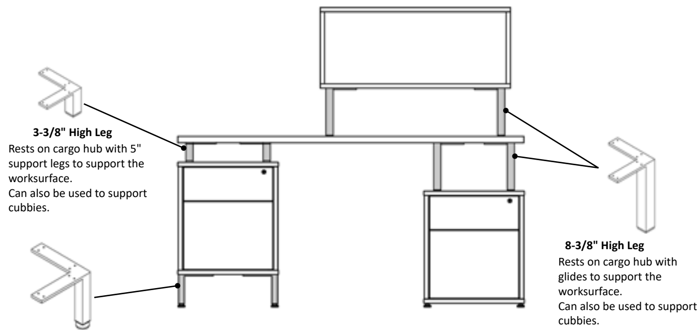
5" High Leg
